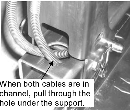
Figure 3. Cable Up From Channel To Support
